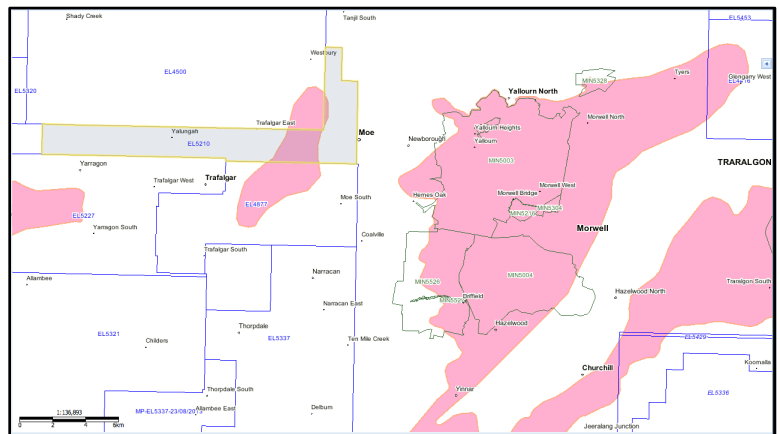
Mantle's EL 5210 and Greenpower's EL's 4500, 4877 and 5227.
